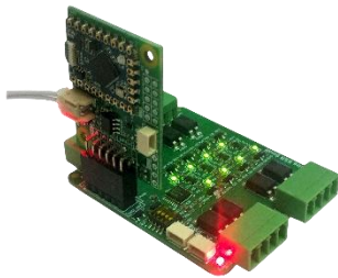
IoTextra SSR Small with a vertically mounted IoTsmart RP2350 module
