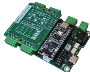
IoTbase Nano with the IoTextra SSR Small module
